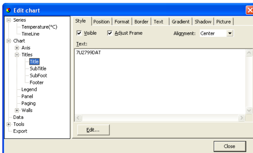
Figure 8.17 Titles Menu
