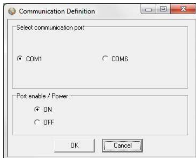
Figure 4.2 Communication Definition
