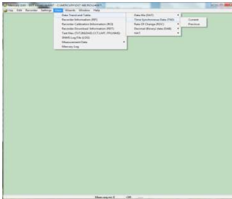
Figure 10.3 Previous Conversions
