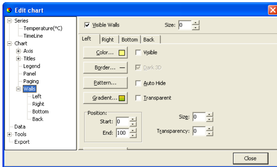
Figure 8.21 Walls Menu
