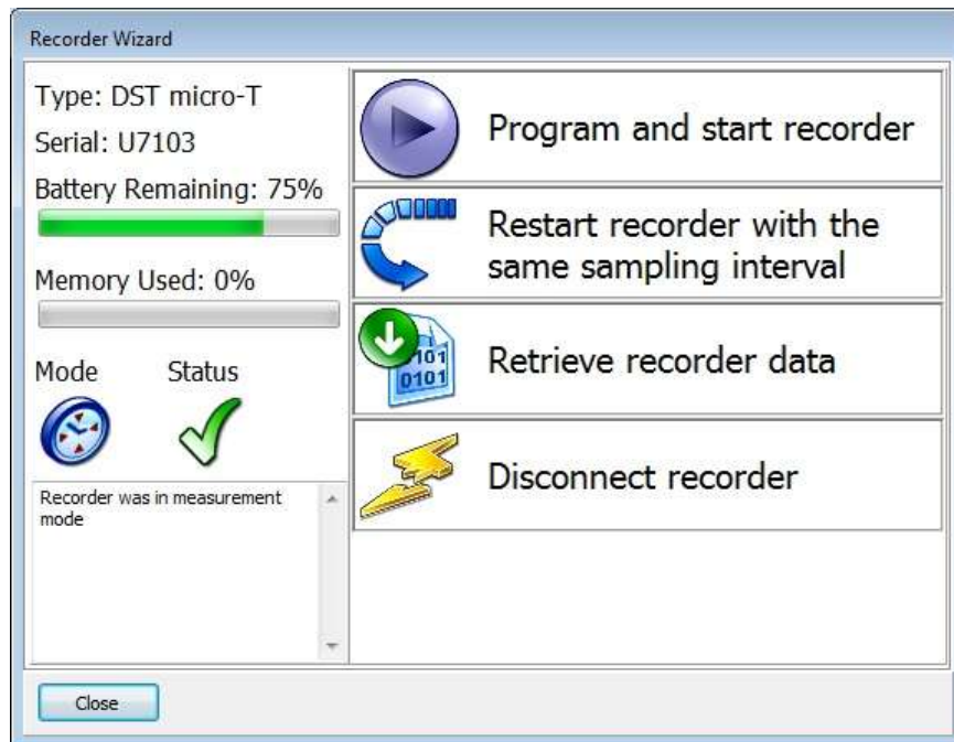
Figure 5.13 Recorder wizard
