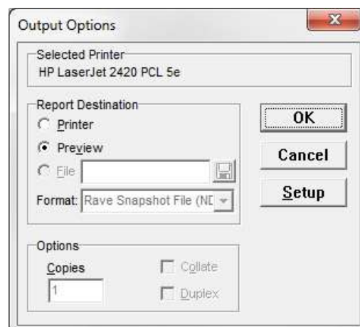
Figure 7.3 Output Options
