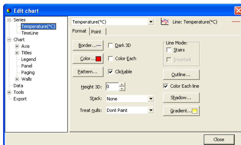
Figure 8.15 Format Series
