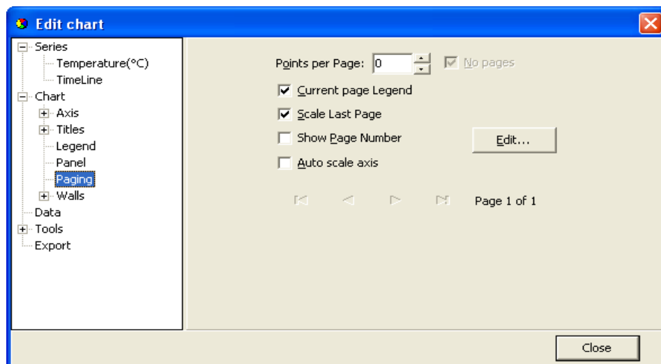
Figure 8.20 Paging Menu
