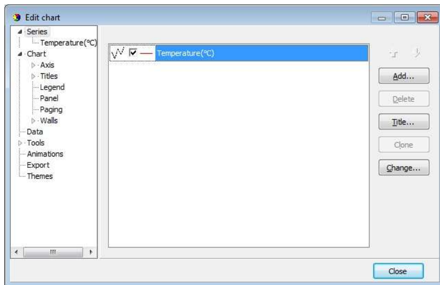
Figure 6.7 Editing Chart
