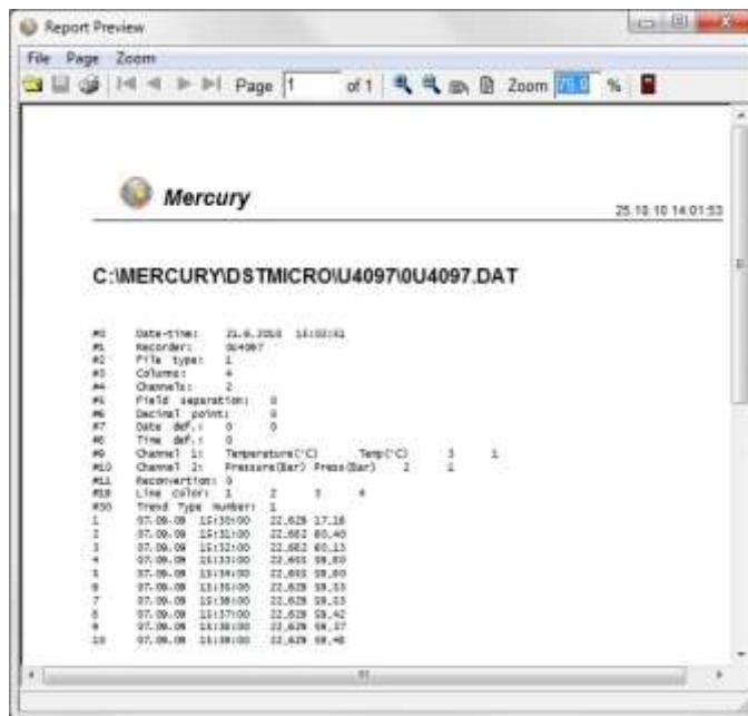
Figure 7.6 Report Preview
