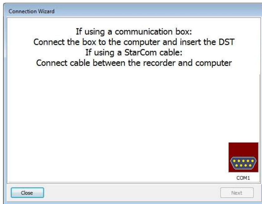
Figure 13.1 Connection Wizard
