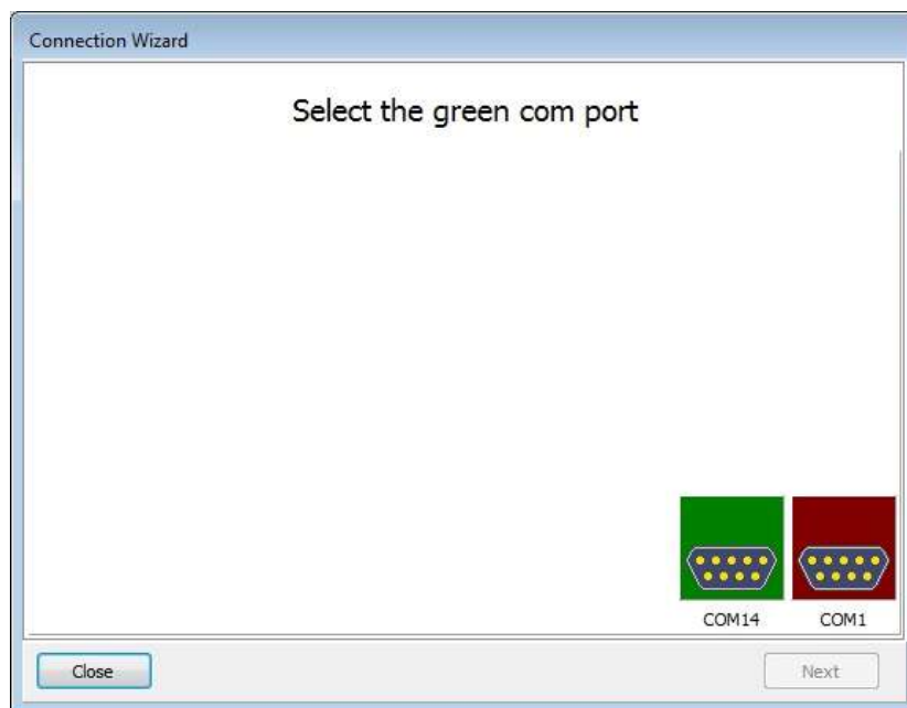
Figure 5.1 Connection Wizard
