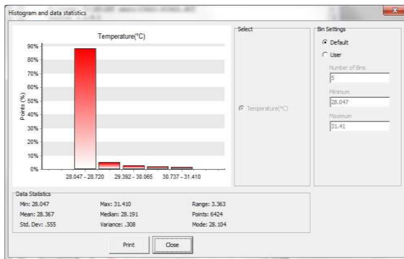
Figure 7.2 Histogram
