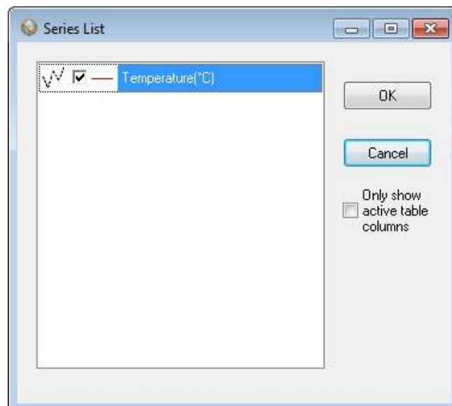
Figure 6.2 Series list
