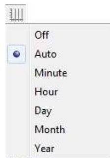
Figure 6.5 vertical gridlines
