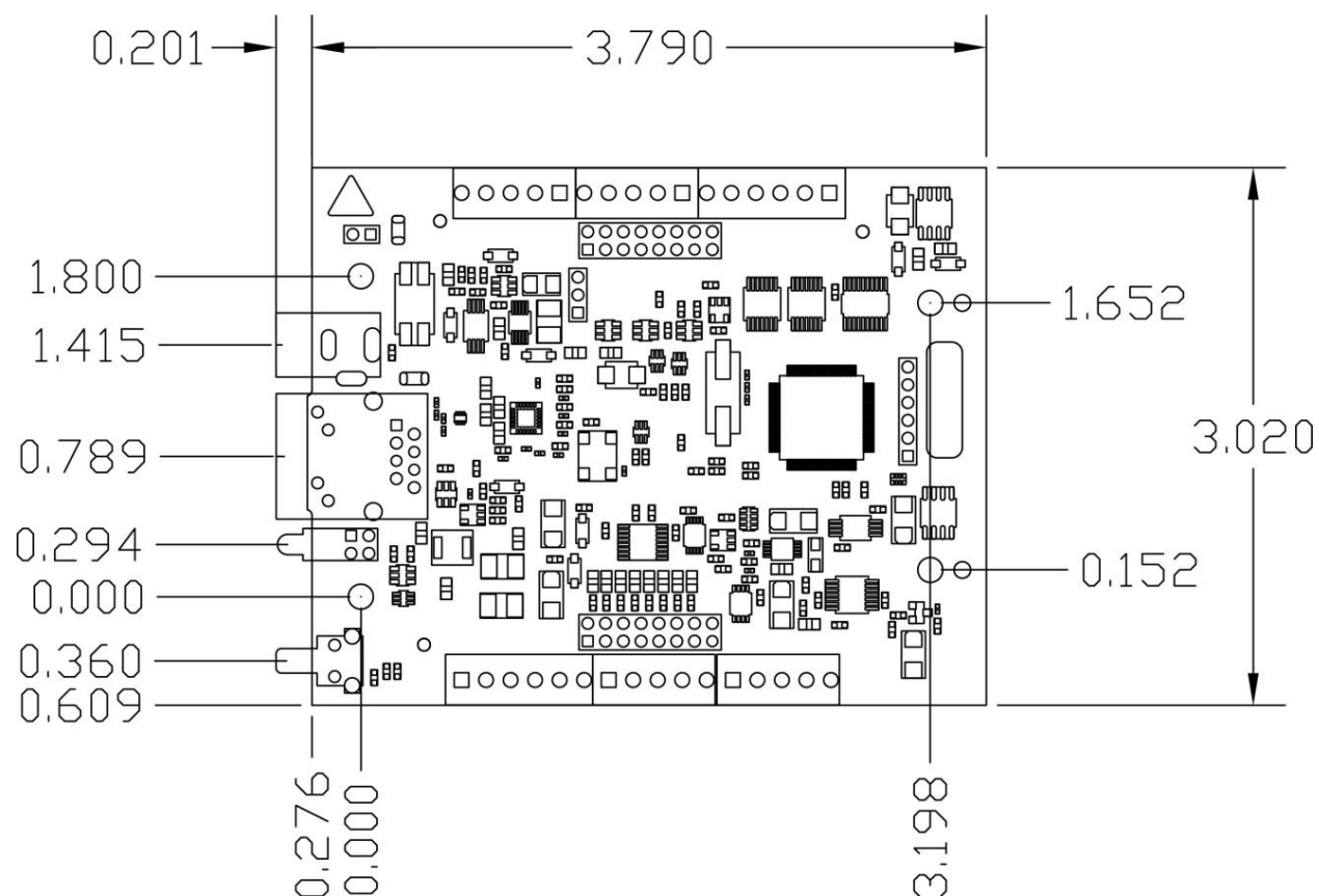
Figure 8. E-1608 device circuit board dimensions
