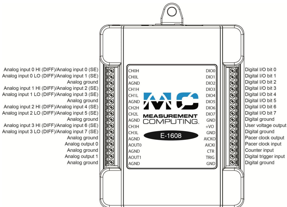
Figure 3. E-1608 pinout
