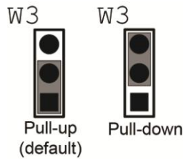
Figure 7. W3 jumper configurations
