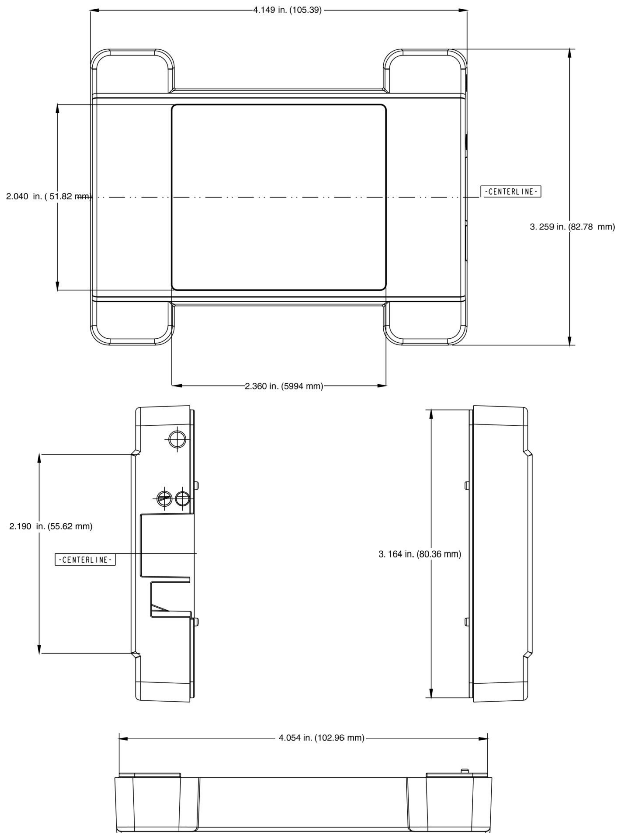
Figure 10. E-1608 top enclosure dimensions
