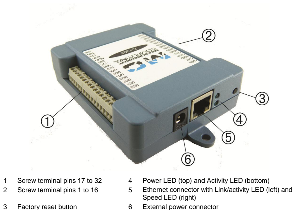
Figure 2. E-1608 external components
