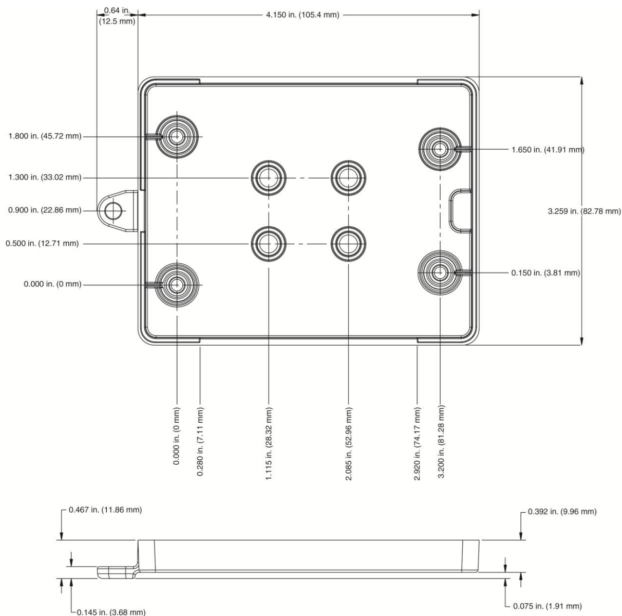
Figure 9. E-1608 bottom enclosure dimensions
